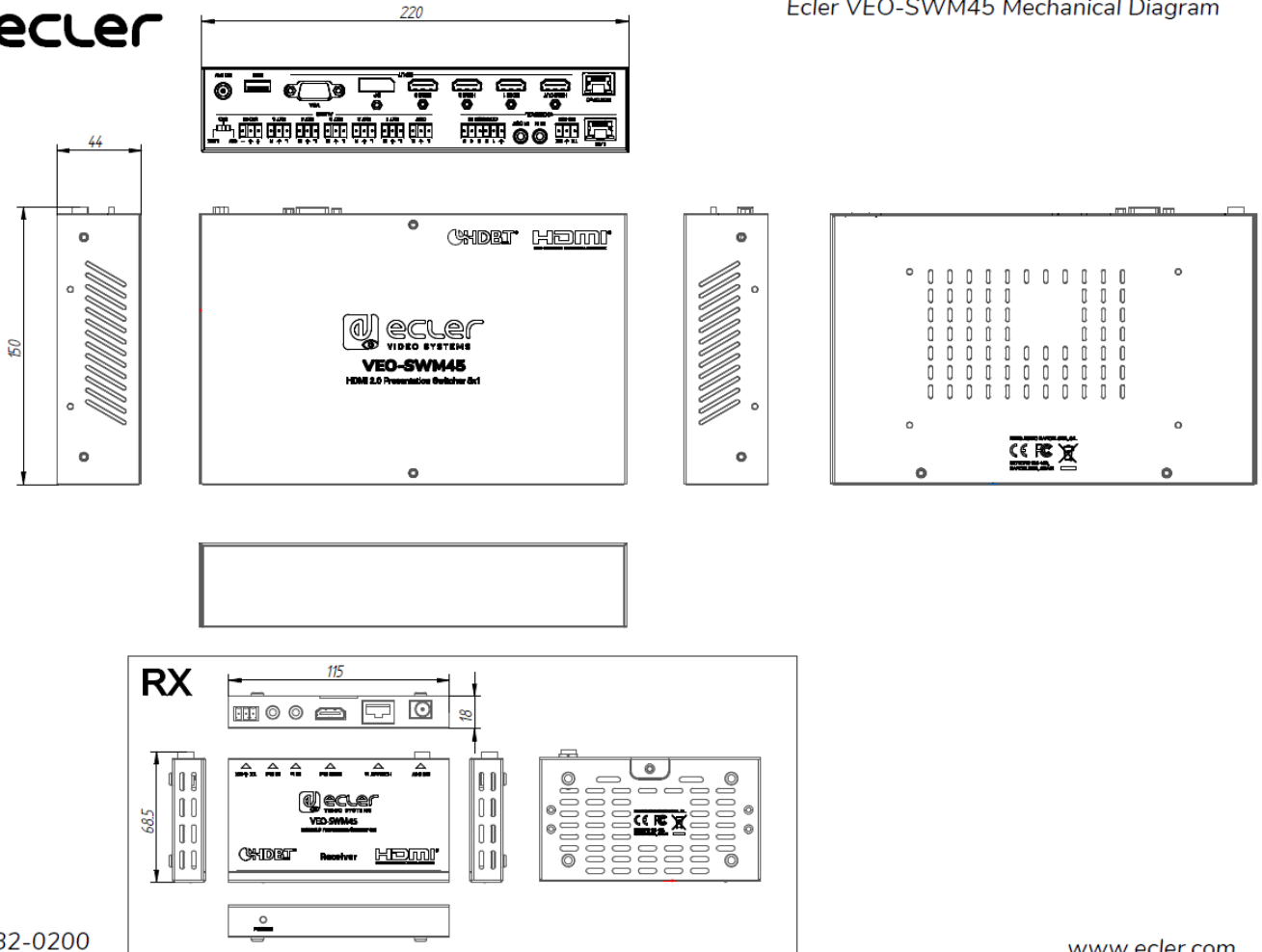
Ecler VEO-SWM45 Mechanical Diagram
