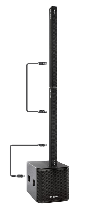
2 x LABI1-C100i + 1 x LABI1-SB18p Mono-double column configuration
