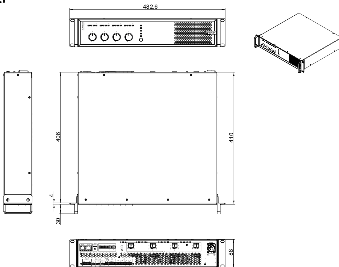
Ecler VIDA-48Q Mechanical Diagram
