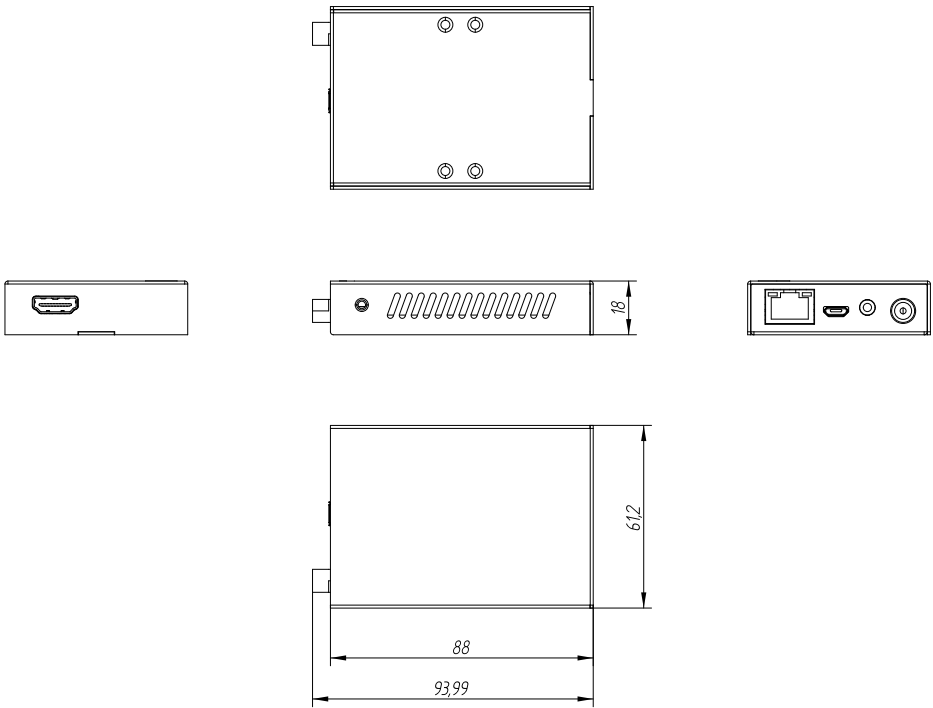
Ecler VE0-SPS4 RX Mechanical Diagram
