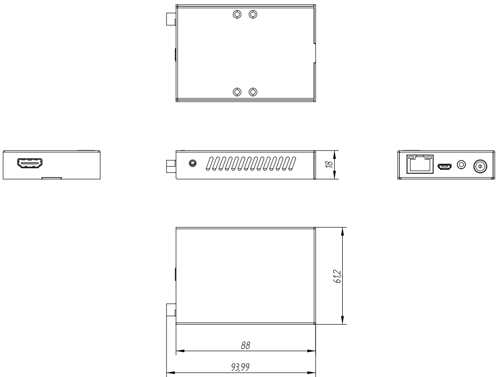
Ecler VE0-SPS4 RX Mechanical Diagram
