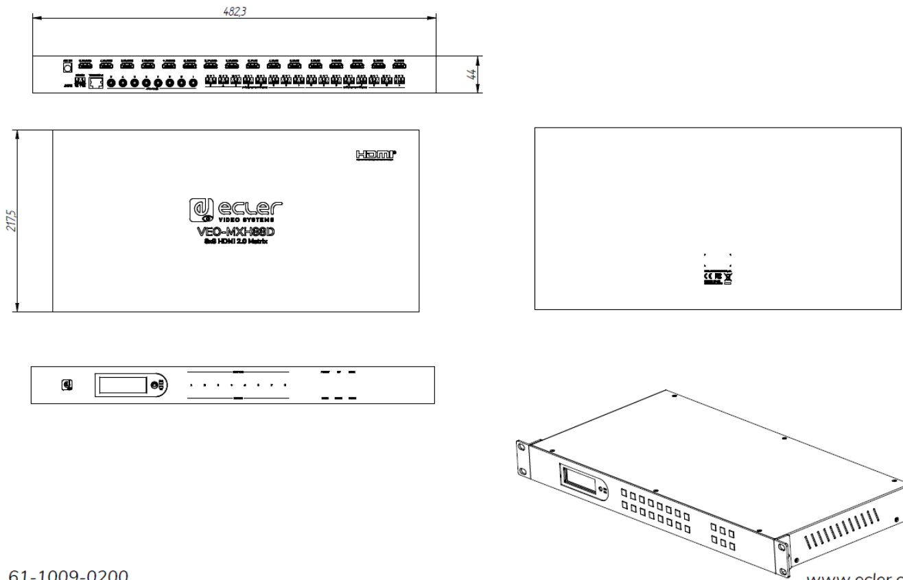
Ecler VEO-MXH88D Mechanical Diagram
