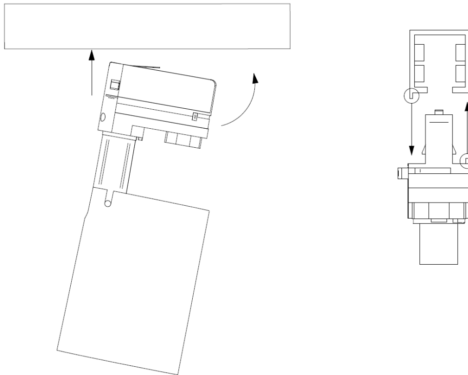
Connection to a GLOBAL Trac Pro / Eutrac lighting rail (three-circuit lighting track system)
