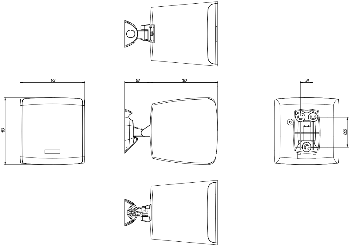
Ecler eMOTUS5OD Mechanical Diagram
