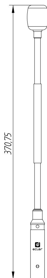
Ecler PAGE-X4 Mechanical Diagram
